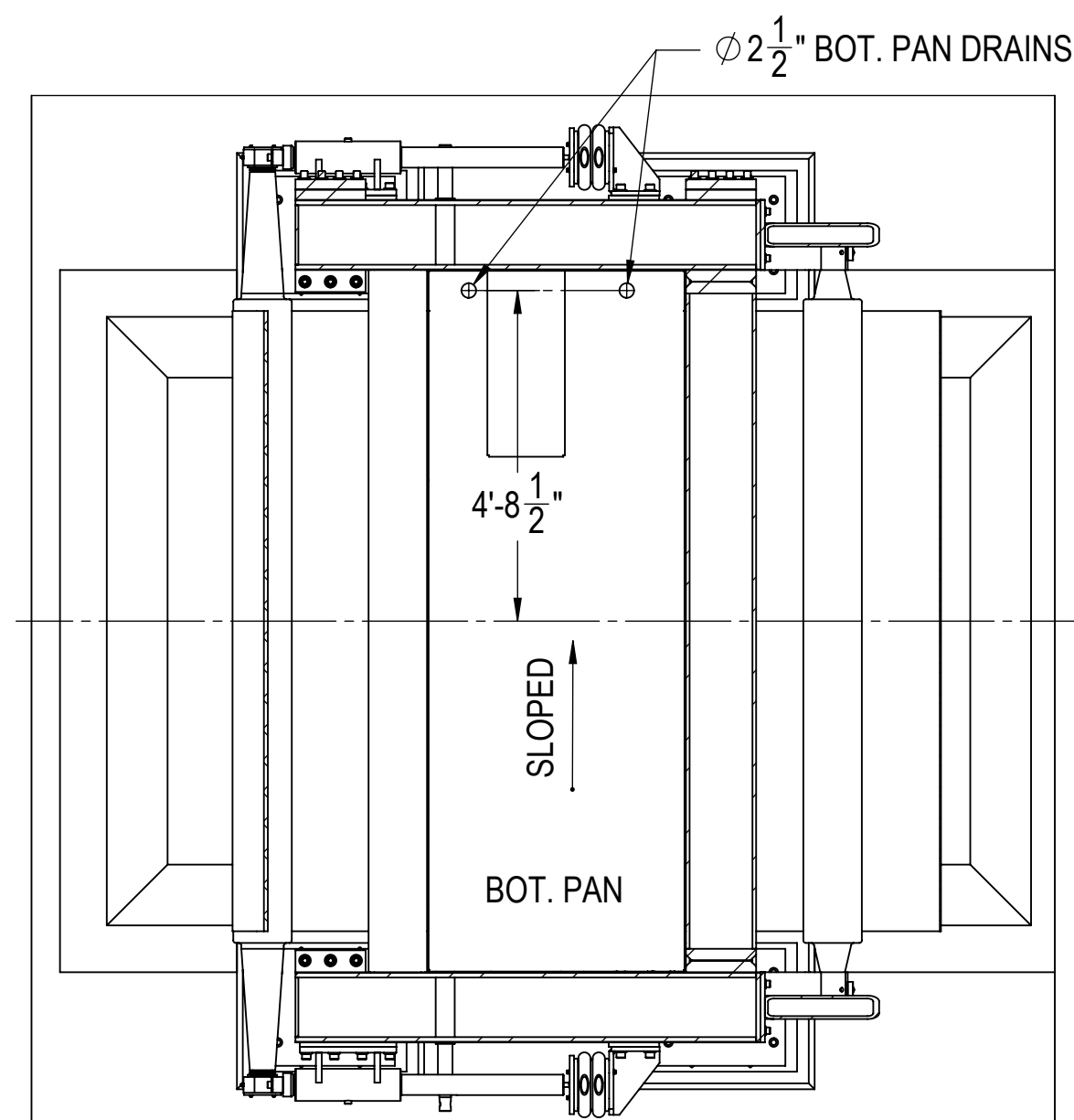
SECTION C-C
